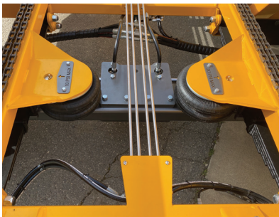
Spring & air bag suspension
